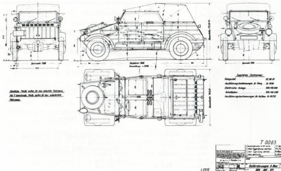
Complete drawings of the Type 82 Kübelwagen.
