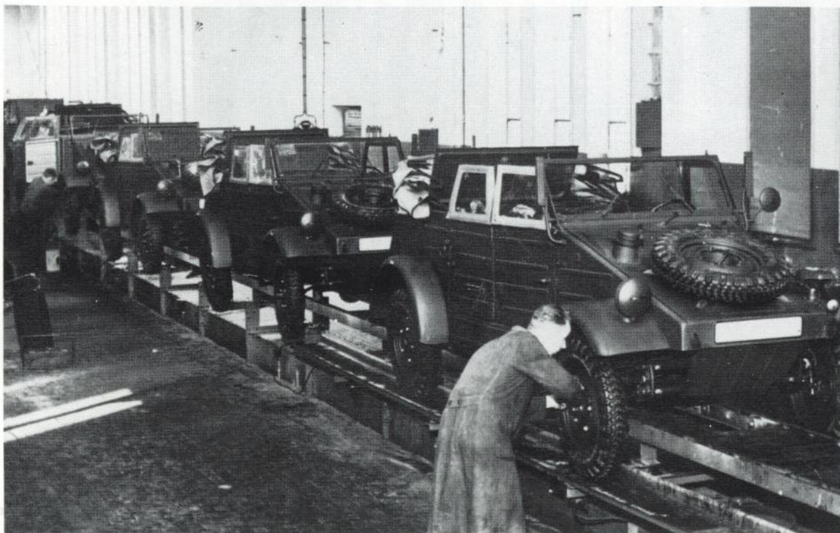
Above: Kübelwagen in the paint drying oven.
